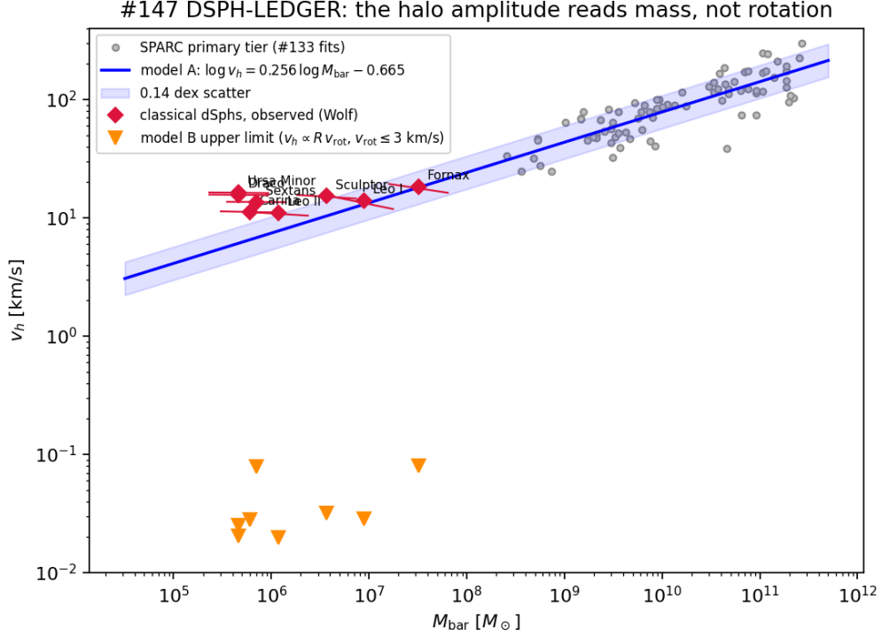
Figure 4: The dwarf-spheroidal ledger ( #147 ). The eight classical dSphs (diamonds; bars span the M_*/L sweep) against the SPARC primary tier (grey) and the measured mass law Eq. (6) (line, with 0.14 dex band). Triangles: the rotation-proportional entrainment upper limits at v_{\text{rot}} \leq 3 km/s — short by \sim 2.7 dex. The halo amplitude tracks mass, not rotation.
